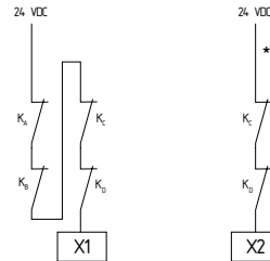
Fig. 7: SRB 400CA, SRB 400CS and SRB 400CA/Q left = switch-off level 1 right = switch-off level 2
